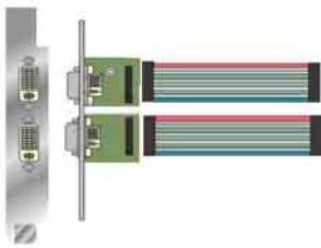
2 DVI module with bracket x 1 (2807750 Serial)
