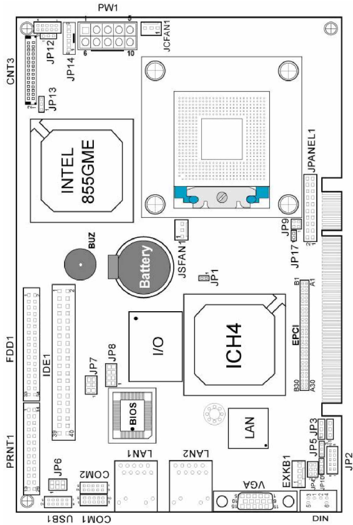
3307560 Connector, Jumper and Component locations
