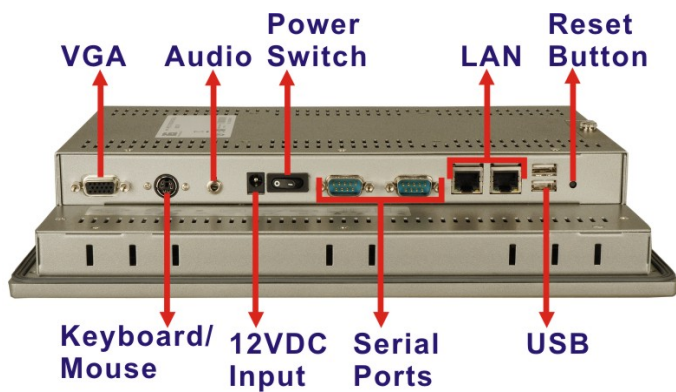
Figure 1-4: 2901190/2901200 Bottom View
