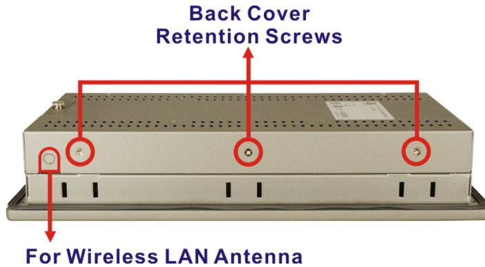
Figure 1-3: 2901190 Top View
