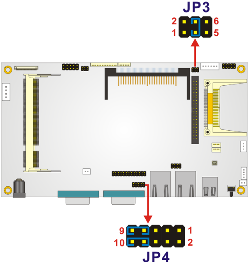
Figure 3-3: Jumper Locations
