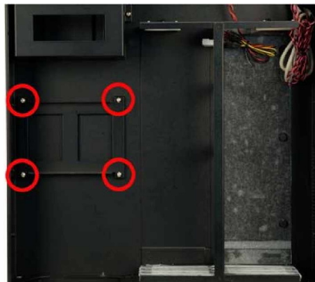
Figure 11: Four Internal 3.5" HDD Bracket Retention Screws
