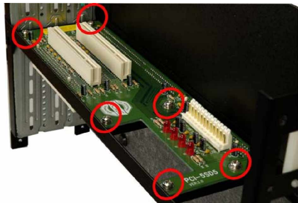
Figure 8: Insert Six Retention Screws
